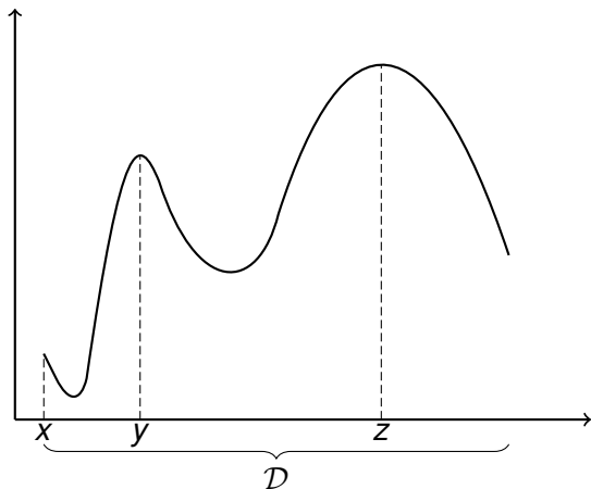
Figure: The points x , y , and z are local maximizers of f on \mathcal{D} ; points y and z are unconstrained local maximizers of f on \mathcal{D} ; while the point z is a (global) unconstrained maximizer of f on \mathcal{D} .
