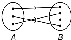
Figure: Injective
