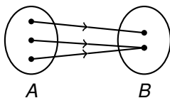
Figure: Surjective
