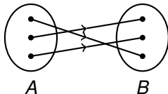
Figure: Bijective
