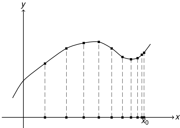
Figure: A continuous function. For any sequence of points (x_n)_{n \in \mathbb{N}} converging to x_0 , the sequence (f(x_n))_{n \in \mathbb{N}} converges to f(x_0) .
