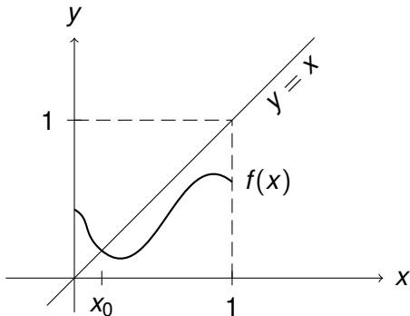
Figure: Fixed point. Kinda obvious?
