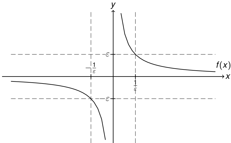
Figure: The function f : \mathbb{R} \setminus \{0\} \rightarrow \mathbb{R} is given by f(x) = 1/x for all x \in \mathbb{R} \setminus \{0\} . The limits at +\infty and -\infty are both 0.
