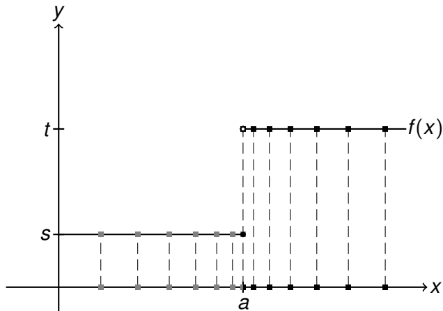
Figure: The right hand limit at a is t , while the left hand limit is s .
