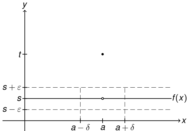
Figure: The (two-sided) limit at a is s , while f(a) = t . (This function is not continuous at a .)
