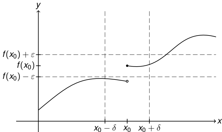
Figure: \epsilon - \delta definition of continuity
